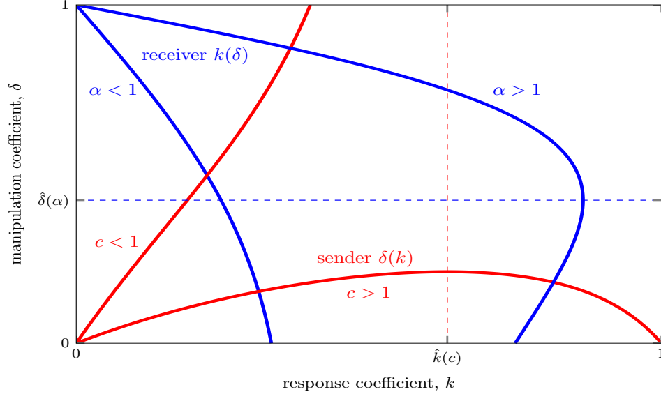
Figure 1: Unique equilibrium.
